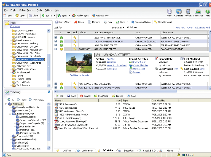
With WinTOTAL's File PowerView, you can track your files easily. See all your orders and reports at once. View, set and send status messages – all in one location.
